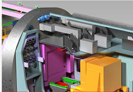
ANDRA CIGEO - Handling process engineering
